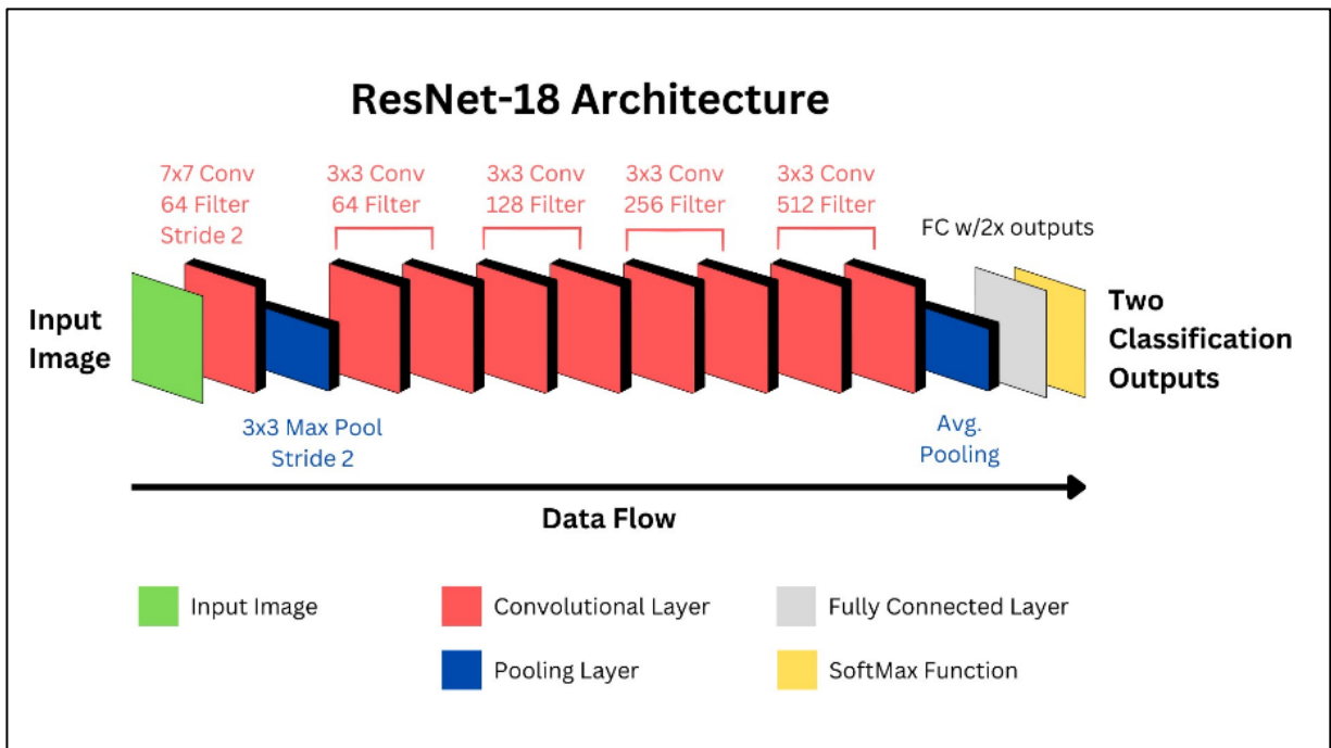
Figure 3.4 Overview of the ResNet 18 model. Adapted from https://arxiv.org/abs/1902.08897
