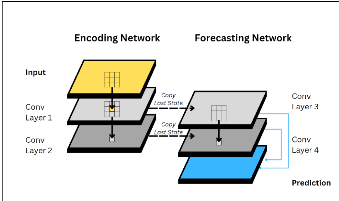
Figure 3.8 Network architecture for the ConvLSTM. The input layer is a 3D representation of a satellite dataset, e.g., an observation at location x, y , and time t . In the encoding network, each layer compresses the input to hidden states (ConvLSTM Layer 1) and hidden state to other hidden states (ConvLSTM Layer 2). In the forecast network, the previous hidden state (ConvLSTM Layer 1 and 2) is copied and decoded (ConvLSTM 3 and 4). Adapted from Shi et al. 2015.
