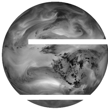
GOES-16 - Channel 08
