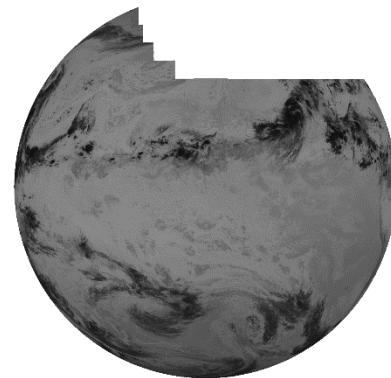
GOES-18 - Channel 13
