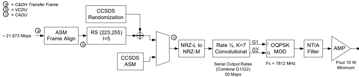
Figure SC-GND-4528. HRD Transmitter Function Block Diagram
