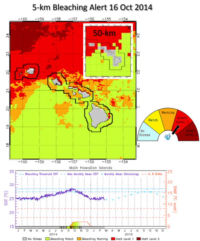
Improved spatial resolution is evident in the 5-km Bleaching Alert during the first-ever mass coral bleaching event in Hawai‘i, derived from NOAA’s Operational Geo-Polar SST, 10/16/14
