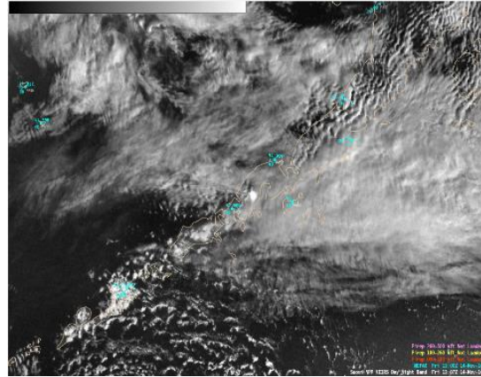
Nighttime images of Suomi NPP VIIRS Day/Night Band of an eruption of the Pavlof Volcano on November 13, 2014.
