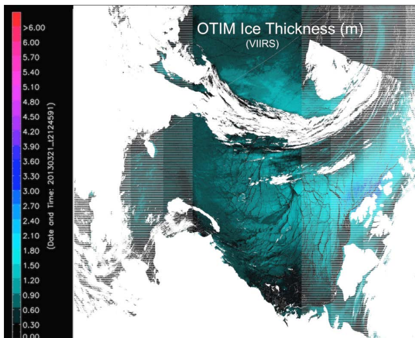
OTIM retrieved ice thickness based on VIIRS data on March 21, 2013
