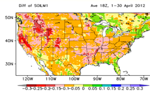
Difference between GFS sensitivity and control runs
