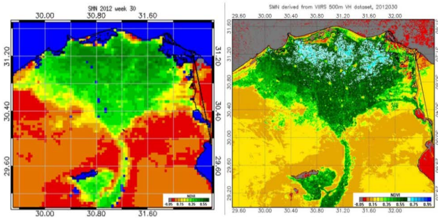
Noise reduced NDVI derived from AVHRR (left, 4km resolution) and VIIRS (right, 500m resolution).
