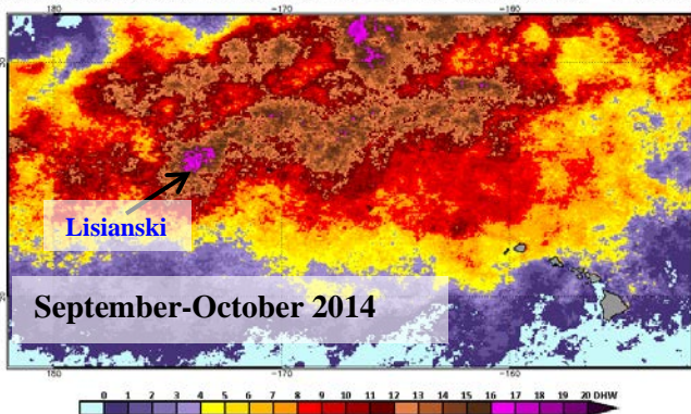
NOAA Coral Reef Watch Daily 5-km Blended Geo-Polar Night-Only Degree Heating Weeks 17 Oct 2014
